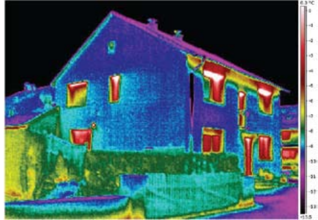
After Insulation with Haacke® insulating Brick
